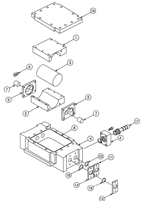
Quantronix Laser Head Components
